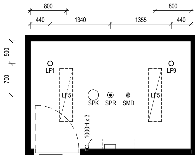
4 RCP - VILLAGE HEALTH & WELLNESS - CONSULT 2 Scale 1: 50
