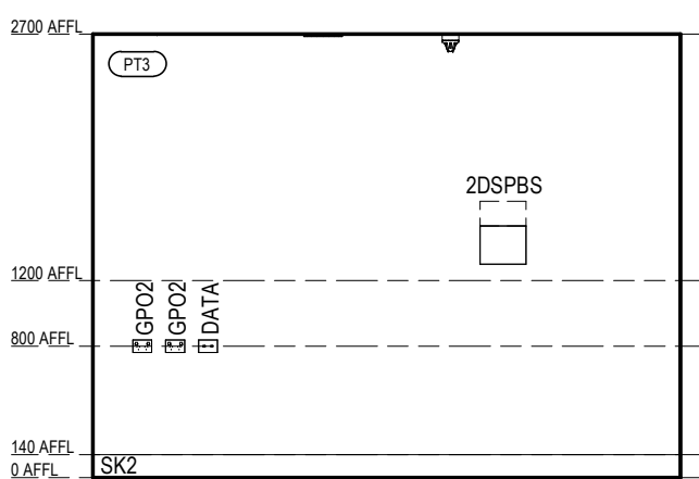
VILLAGE HEALTH & WELLNESS - CONSULT 2 ELEVATION 1 Scale 1: 50
