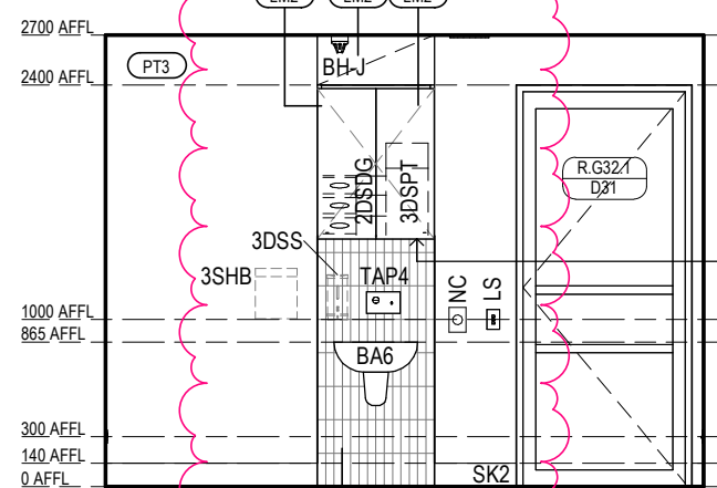
VILLAGE HEALTH & WELLNESS - CONSULT 2 ELEVATION 3 Scale 1: 50
