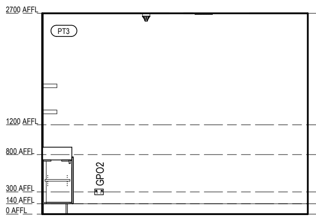
VILLAGE HEALTH & WELLNESS - CONSULT 1 ELEVATION 1 Scale 1: 50
