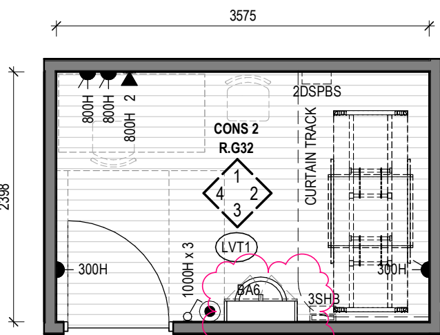
3 VILLAGE HEALTH & WELLNESS - CONSULT 2 Scale 1: 50
