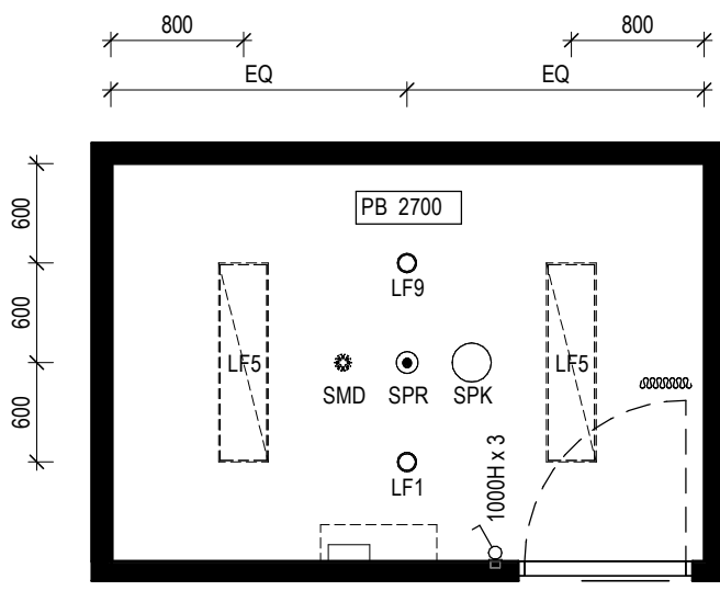
2 RCP - VILLAGE HEALTH & WELLNESS - CONSULT 1 Scale 1: 50
