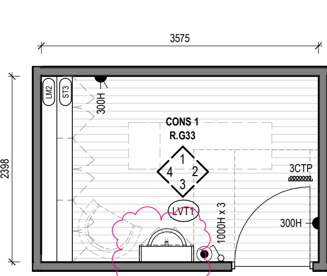
1 VILLAGE HEALTH & WELLNESS - CONSULT 1 Scale 1: 50
