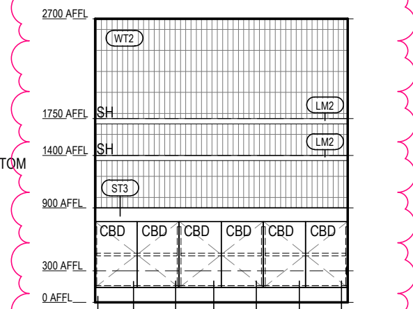
VILLAGE HEALTH & WELLNESS - CONSULT 1 ELEVATION 4 Scale 1: 50
